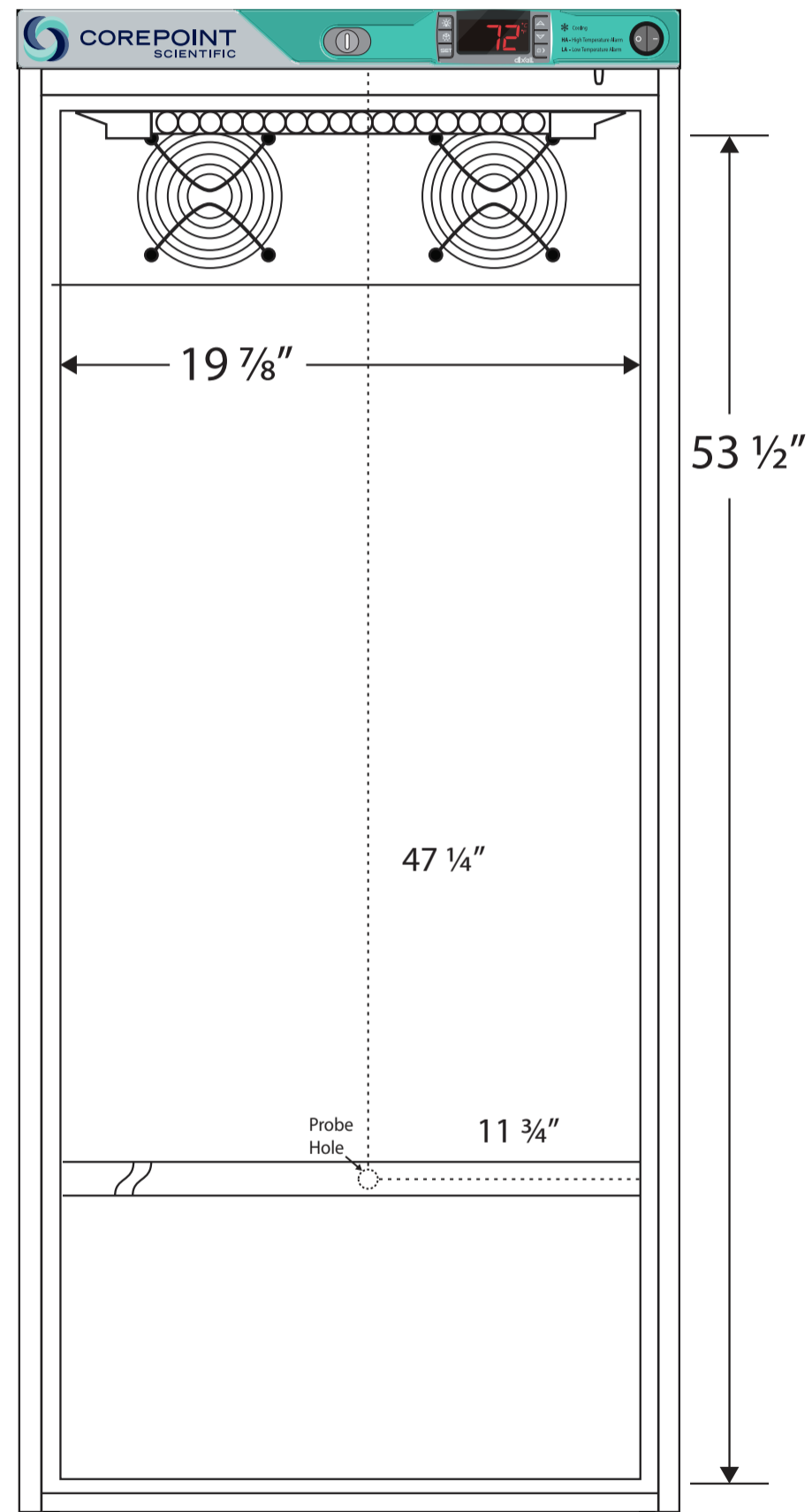
Front View
