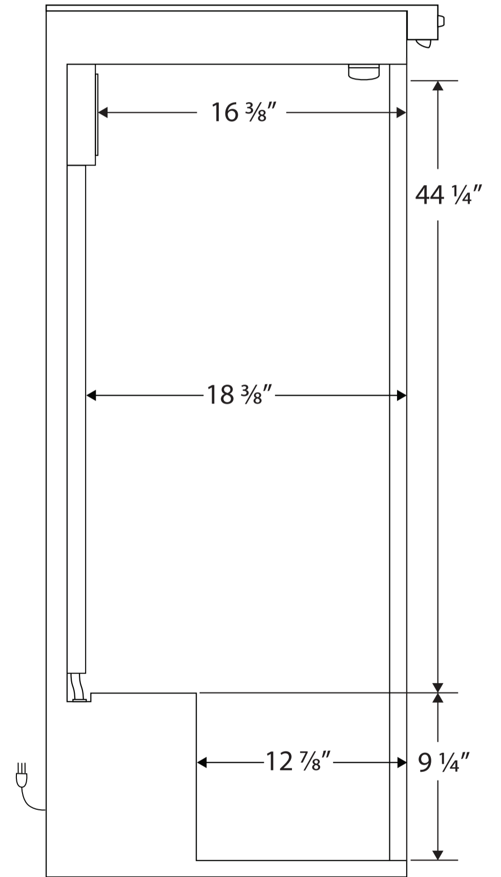
Side View
